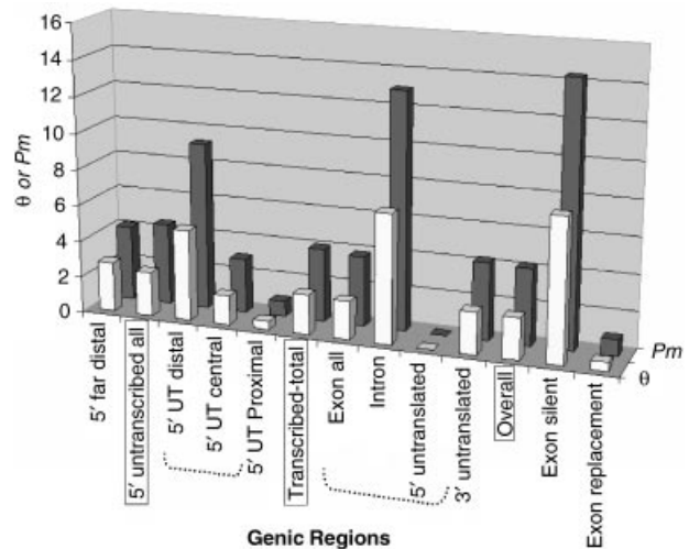
Fig. 3 Polymorphicity ( Pm ) and the population mutation rate ( \theta ) of various genic regions of the Est-6 gene of Drosophila simulans (data modified from Karotam et al. 1995). Columns in the front row are \theta -values; columns at the back are Pm . It can be seen that Pm and \theta are highly correlated. As shown in the figure, from left to right, a gene can be divided into 5' far distal region, 5' untranscribed region (which can further be fragmented to distal, central and proximal regions), and transcribed region (which comprises exons, introns, 5' untranslated and 3' untranslated regions) (see Box 2). 'Overall' refers to a gene as a whole, 'exon silent' and 'exon replacement' refer to the total of silent sites and replacement sites in all exons, respectively.
