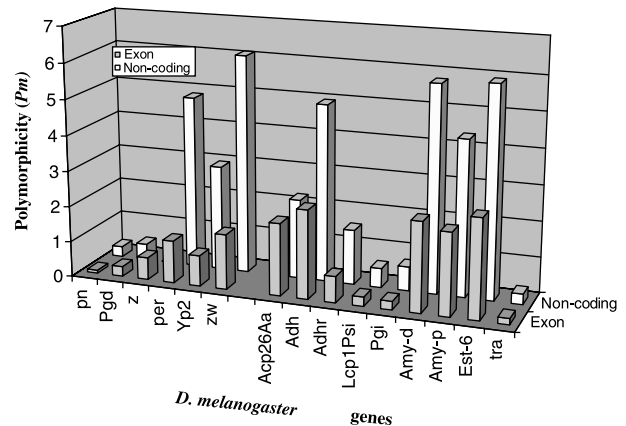
Fig. 2 Polymorphicity ( Pm ) of exon and noncoding regions of 15 D. melanogaster genes, of which six are X chromosome-linked genes and nine autosomal genes (data modified from Moriyama & Powell 1996). Pm of noncoding regions (light columns), which is largely contributed by introns, is clearly higher than that of exons (dark columns).
