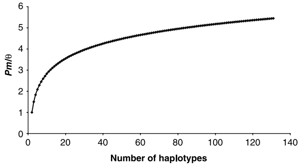
Fig. 1 Effect of the number of haplotypes sampled from populations on the correlation of Pm (the 'polymorphicity') and \theta (the estimated population mutation rate, or the heterozygosity). See text for the definition of Pm .
